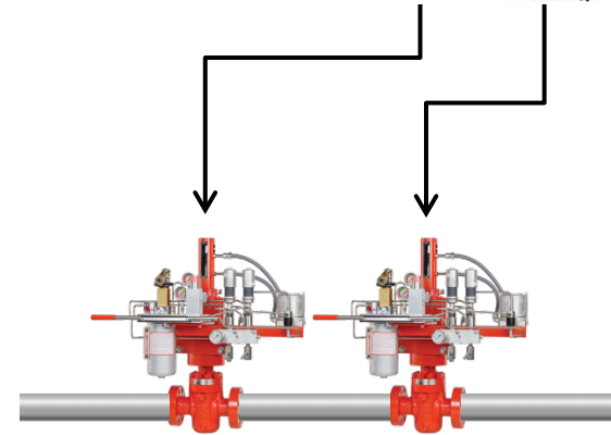
ESD Valves
